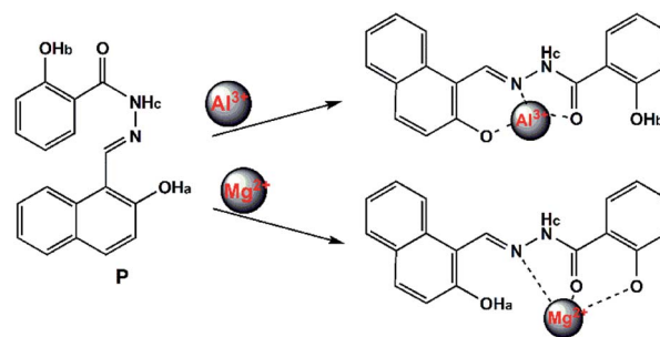
Scheme 2 Proposed binding modes of P with \text{Al}^{3+} and \text{Mg}^{2+} .
