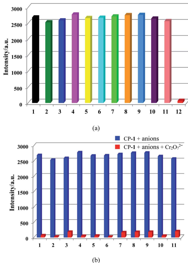
Fig. 5 Luminescence intensity histograms of CP-1 (1 mg) dispersed into various anion aqueous solutions ( 2 \text{ mL}, 10^{-3} \text{ M} ) excited at 278 \text{ nm} (a) and subsequent addition of \text{Cr}_2\text{O}_7^{2-} (b). (1) Blank, (2) \text{F}^- , (3) \text{Cl}^- , (4) \text{Br}^- , (5) \text{I}^- , (6) \text{CH}_3\text{COO}^- , (7) \text{SO}_4^{2-} , (8) \text{H}_2\text{PO}_4^- , (9) \text{ClO}_4^- , (10) \text{SO}_3^{2-} , (11) \text{SCN}^- , (12) \text{Cr}_2\text{O}_7^{2-} (b).
