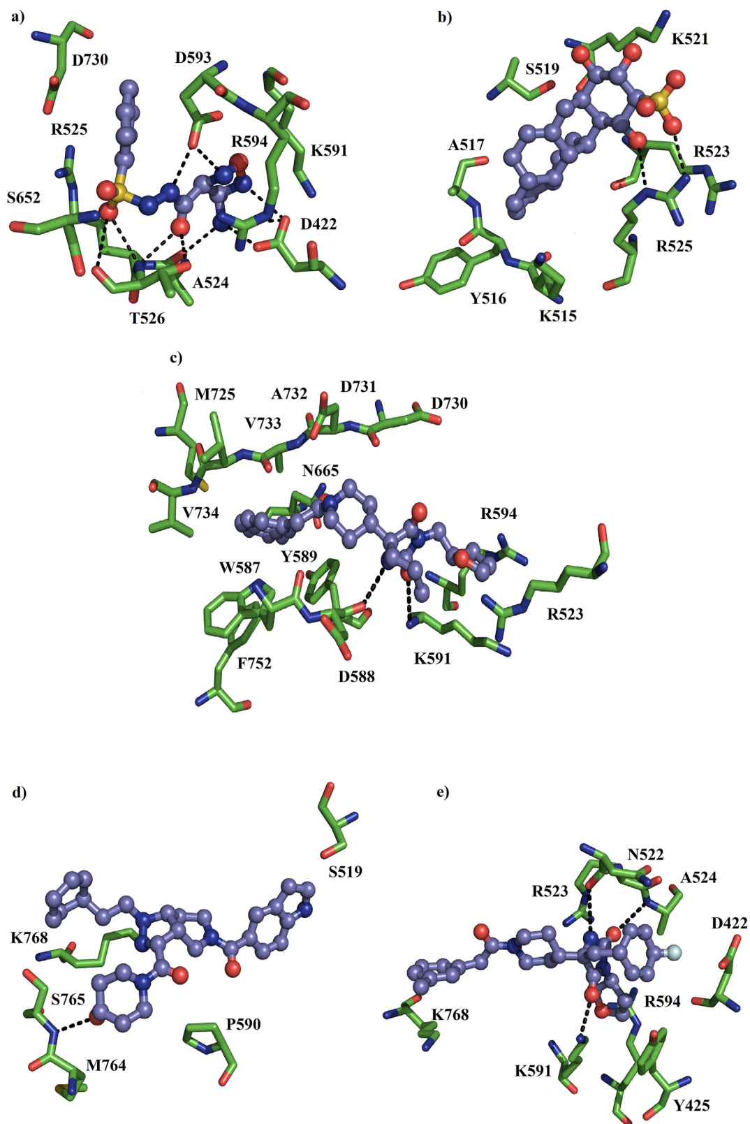
Figure 4. The binding orientation of 5 best ligands inside the receptor binding site of SARS Cov-2 RdRp. a) ZINC000005605139, b) ZINC000006094731, c) ZINC000012161475, d) ZINC000014751834 and e) ZINC000014882040. The binding orientation indicates stable binding for each of the 5 ligands to the RdRp of Cov-2.
