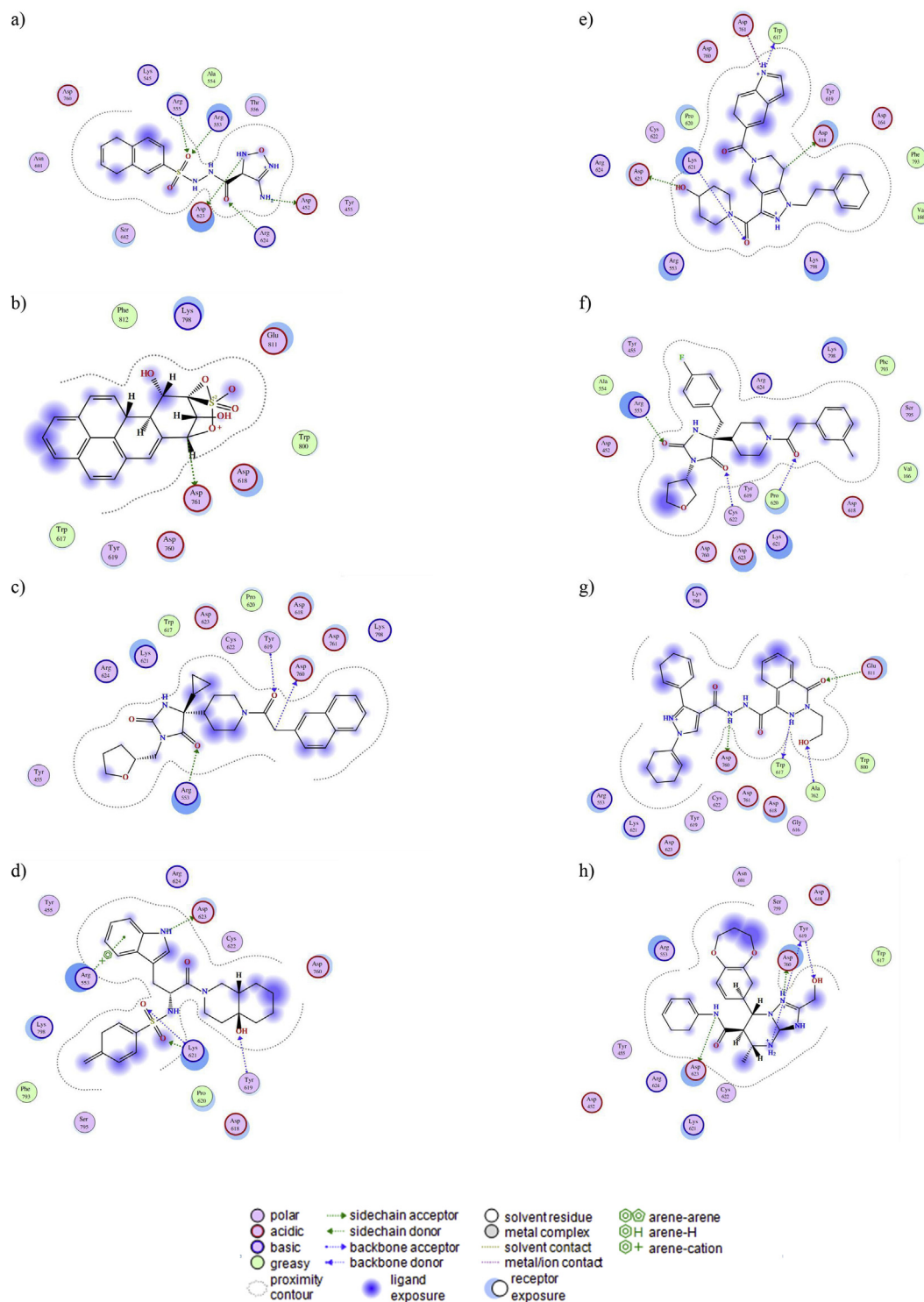
Figure 2. Molecular docking of probable inhibitory molecules onto RdRp. Panels (a–h) show the 2D structures of the binding interaction of the ligands inside the pocket of SARS-Cov-2 RdRp a) ZINC000005605139, b) ZINC000006094731, c) ZINC000012161475, d) ZINC000014751834 and e) ZINC000014882040, f) ZINC000012863240, g) ZINC000049581065, h) ZINC000072460420. The types of interaction are shown at the end of the figure.
