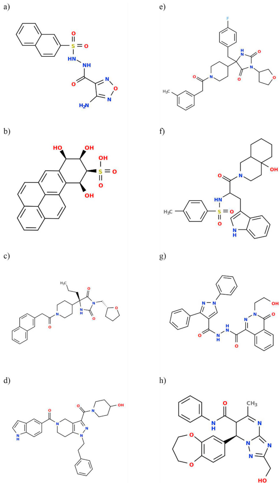
Figure 1. The chemical structures of ligands that were selected based on the initial virtual screen. a) ZINC000005605139, b) ZINC000006094731, c) ZINC000012161475, d) ZINC000014751834 and e) ZINC000014882040, f) ZINC000012863240, g) ZINC000049581065, h) ZINC000072460420.
