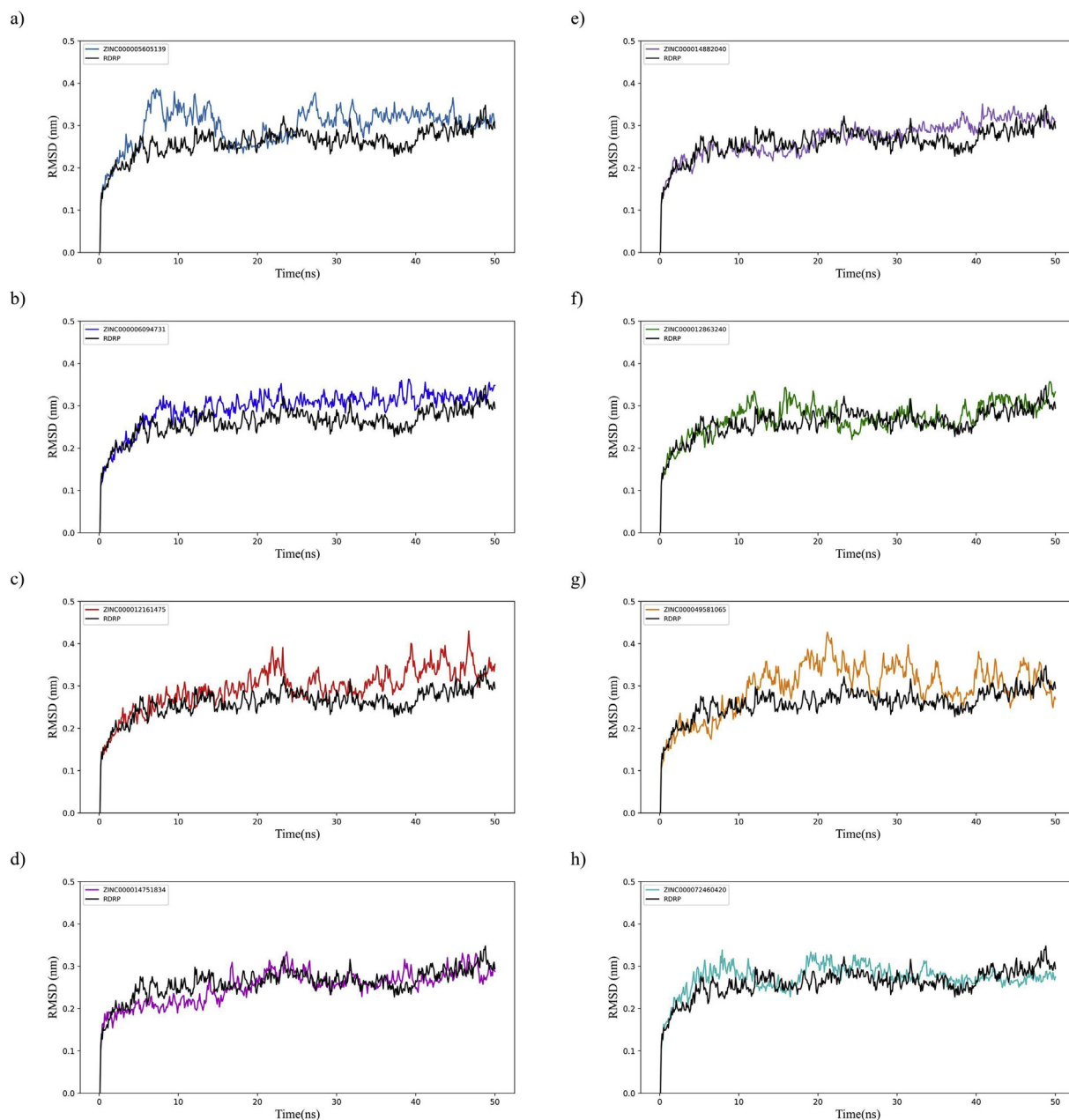
Figure 3. RMSD pattern of docked complexes compared to Cov-2 RdRp. a) ZINC000005605139, b) ZINC000006094731, c) ZINC000012161475, d) ZINC000014751834 and e) ZINC000014882040, f) ZINC000012863240, g) ZINC000049581065, h) ZINC000072460420. The RMSD pattern show that all the small molecules docked to the RdRp protein remain relatively stable under the simulated environment.
