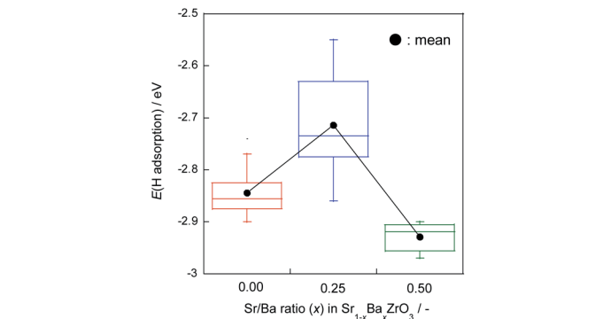
Fig. 1 Box plots for H atom adsorption energies over \text{Sr}_{1-x}\text{Ba}_x\text{ZrO}_3 ( x = 0.00, 0.25, 0.50 ) oxides. Whisker length is set as 1.5 times of interquartile range. Black plots show mean values.
