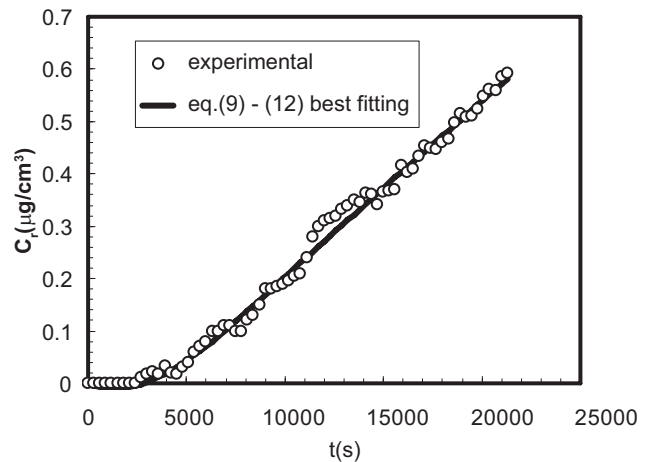
Figure 6 Comparison between experimental data (open circles) referring to single-stranded DNA oligonucleotides release from poly(DL-lactide-co-glycolide) (PLGA) microparticles and subsequent permeation through the synthetic membrane and model best fitting (eq.(9) – (12), solid line). C_r indicates single-stranded DNA oligonucleotides concentration in the receiver chamber.
