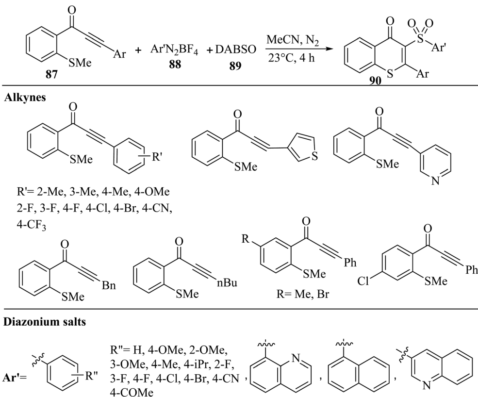
Scheme 39 Synthesis of 3-arylsulfonylated thioflavone derivatives 90 by alkyl-substituted alkyne derivatives. 57
