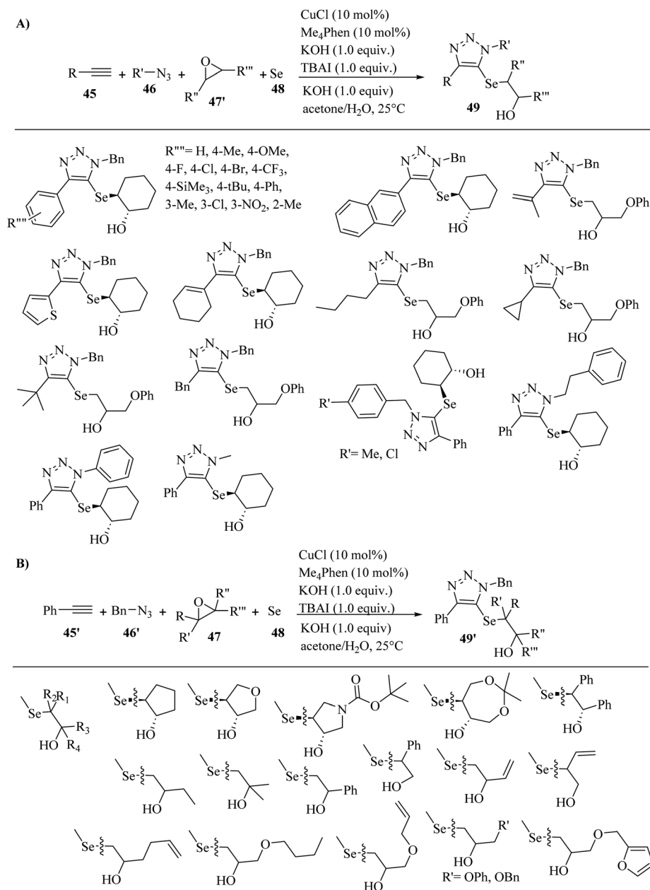
Scheme 19 Synthesis of triazole derivatives using \text{CuCl} catalyst. (A) Substrate scope of alkyne derivatives and azide derivatives. (B) Substrate scope of epoxide derivatives. 41
