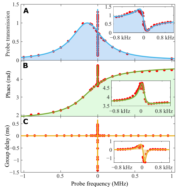
Fig. 5. The probe transmission and group delay modified by a strong control field. (A) Probe transmission as a function of probe frequency ( \Omega_p/2\pi ), including theoretical results (solid lines) and calibrated data (dots). Both a peak and a dip are present in a given control detuning. (B) The phase response of probe transmission. Alteration of phase at \Omega_p \approx 0 signifies strong cavity dispersion. (C) Group delay of probe transmission. A positive value of delay implies a slow light effect, while a negative one implies causality-preserving superluminal effect. P_{\text{con}} \approx 90 \text{ mW} and \Delta_0 \approx 0.28 \kappa are used for all panels.
