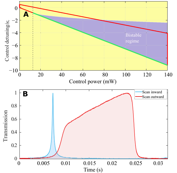
Fig. 2. Stability of the system induced by the photothermal effects. (A) The stability map of the system, with the blue region being the bistability and yellow region being single stability. The parameter regime enclosed with solid curves corresponds to the one of Fig. 6. The green line represents the transition between single stability and bistability. (B) Experimental observation of optical bistability induced by the photothermal effects. At a control power of 160 mW, the cavity response depends on the scanning direction. We observe the self-locking effect when moving the cavity mirror outward and anti-self-locking effect when moving the mirror inward.
