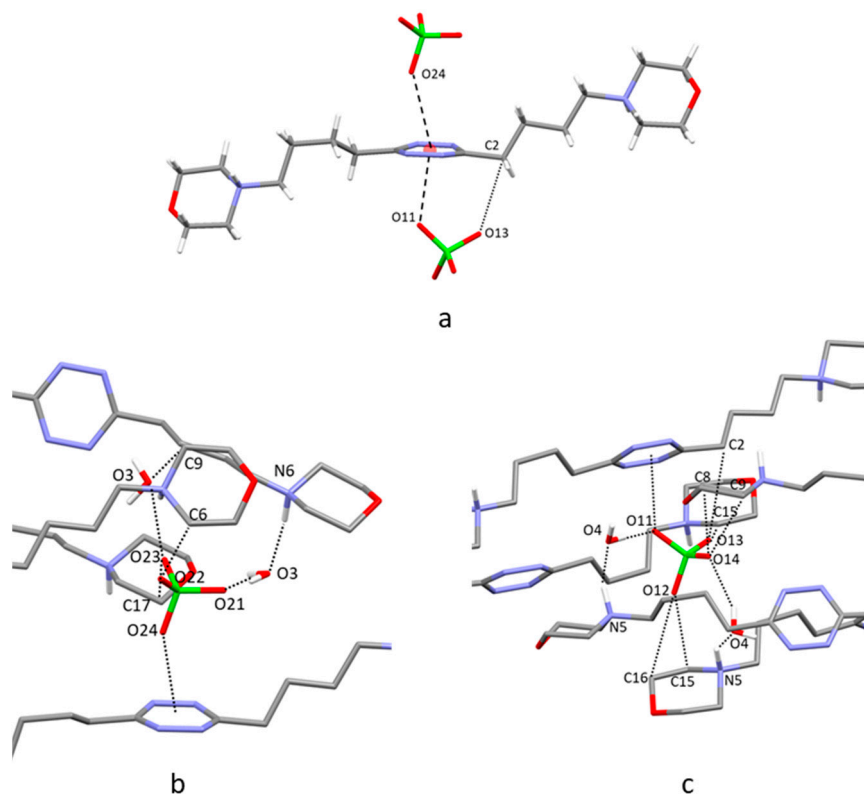
Figure 4. (a) Anion– \pi interactions in the crystal structure of \text{H}_2\text{L4}(\text{ClO}_4)_2 \cdot 2\text{H}_2\text{O} . (b,c) Interactions established by \text{ClO}_4^- ions in the pockets formed by the symmetry-related ligands and the cocrystallized water molecules.
