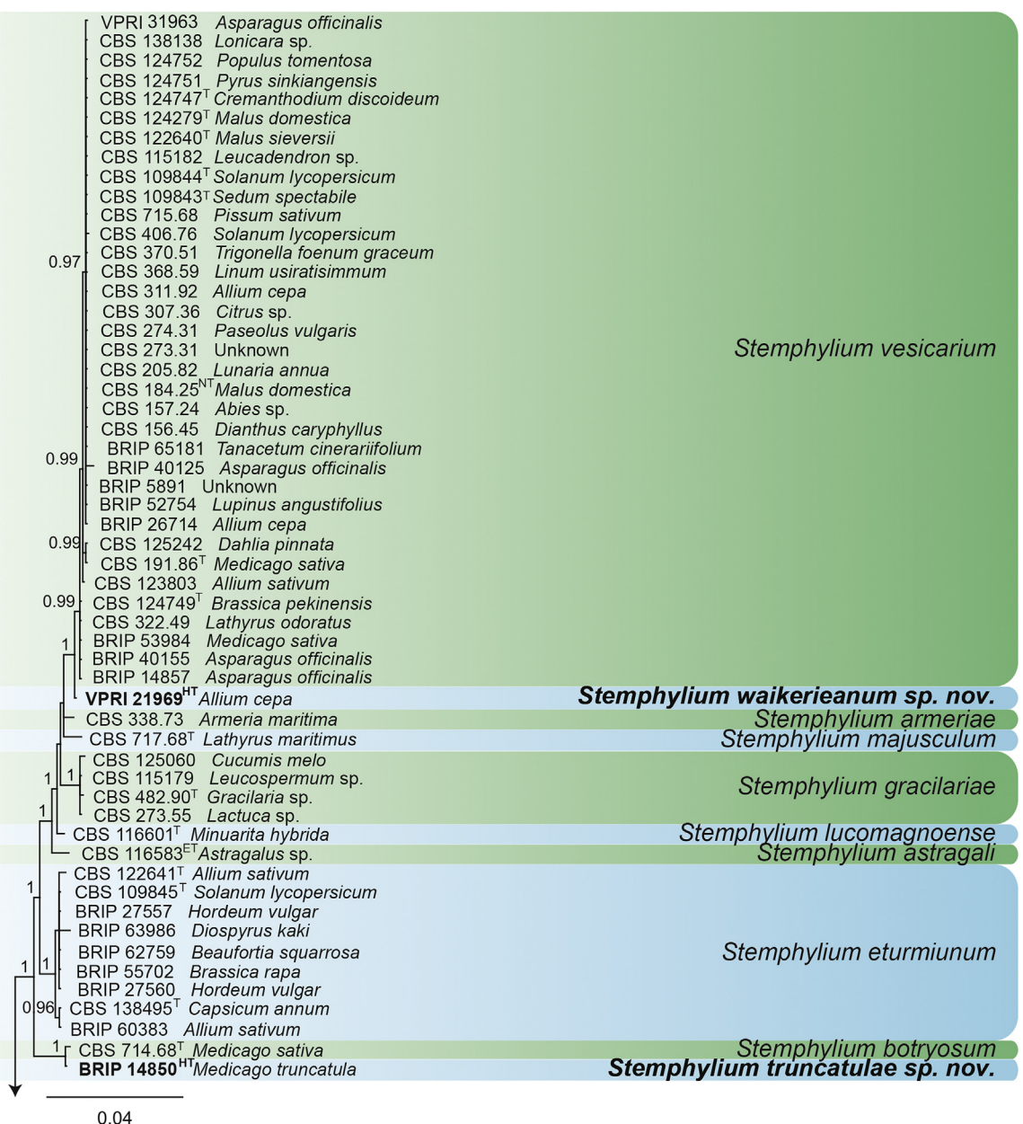
Fig. 78. Bayesian phylogenetic tree inferred from ITS (565 bp), gapdh (613 bp) and cmdA (863) using partitioned analysis with N92+G+I substitution model for ITS and gapdh and GTR+G+I for cmdA . Highest log likelihood -34098.05. The analysis involved 122 nucleotide sequences including 98 sequences obtained from GenBank and 24 sequences obtained in the present study. Scale bar indicates expected changes per site. The tree was rooted to Alternaria alternata (GV14 634a1). The novel species described in this study are shown in bold . Bayesian posterior probability scores above 0.95 are shown at the nodes. GenBank accession numbers are indicated in Table 20. T , ET , HT and NT indicate ex-type, ex-epitype, ex-holotype and ex-neotype strains, respectively. TreeBASE:S23794.
