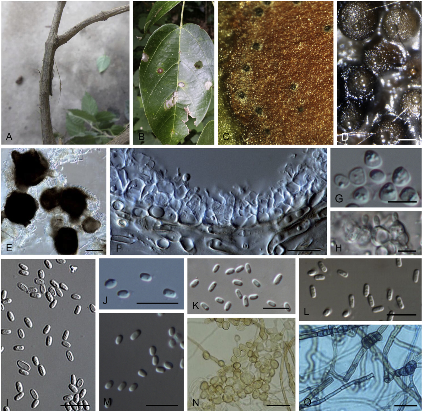
Fig. 1. Allohoma spp. A, B. Disease symptoms. A. Symptoms caused by Allohoma hayatii (ex-type CBS 142859) on Lantana camara . B. Symptoms caused by Allohoma pterospermicola (ex-type CGMCC 3.19245) on Pterospermum xylocarpum . C–O. Asexual morph. C. Conidiomata of Allohoma pterospermicola (LC12181) sporulating on Maesa montana . D. Conidiomata of Allohoma oligotrophica (ex-type CGMCC 3.18114) sporulating on OA. E. Conidiomata of Allohoma minor (ex-type CBS 325.82). F. Section of the conidiomatal wall of Allohoma minor (ex-type CBS 325.82). G, H. Conidiogenous cells. G. Allohoma piperis (ex-epitype CBS 268.93). H. Allohoma oligotrophica (ex-type CGMCC 3.18114). I–M. Conidia. I. Allohoma minor (ex-type CBS 325.82). J. Allohoma piperis (ex-epitype CBS 268.93). K. Allohoma oligotrophica (ex-type CGMCC 3.18114). L. Allohoma cylindrispora (ex-type CBS 142453). M. Allohoma nicaraguensis (ex-type CBS 506.91). N. Swollen cells of Allohoma hayatii (ex-type CBS 142859). O. Chlamydospores of Allohoma hayatii (ex-type CBS 142859). Scale bars: D, E = 100 µm; O = 50 µm; N = 20 µm; F, I–M = 10 µm; G, H = 5 µm. Pictures A, N–O taken from Babaahmadi et al. (2018) ; D, H, K, from Chen et al. (2017) ; E, F, I from Aveskamp et al. (2010) ; G, J, M from Chen et al. (2015) ; L from Valenzuela-Lopez et al. (2018) .
