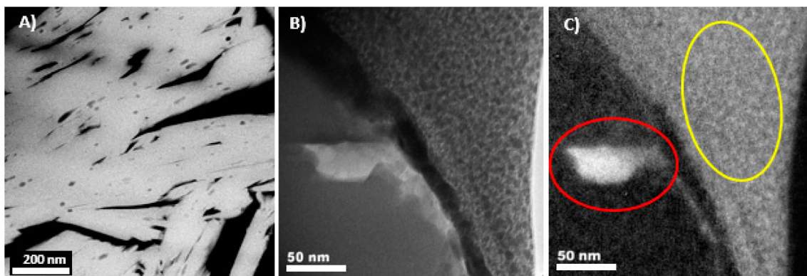
Figure 6. (A) HAADF images in scanning transmission electron microscopy (STEM) mode showing the co-occurrence of C (dark inclusions) within the uranyl vanadate from the Blue Gap Tachee Claim 28 mine waste. (B) Bright-field TEM image and (C) energy filtered transmission electron microscopy (EFTEM) image carbon map confirming that the inclusion in the uranyl vanadate is carbon-rich. The area in red is a C-rich inclusion and the area in yellow indicates carbon retained in the organometallic Pt compound that is used to protect the FIB section from ion beam damage during sample preparation.
