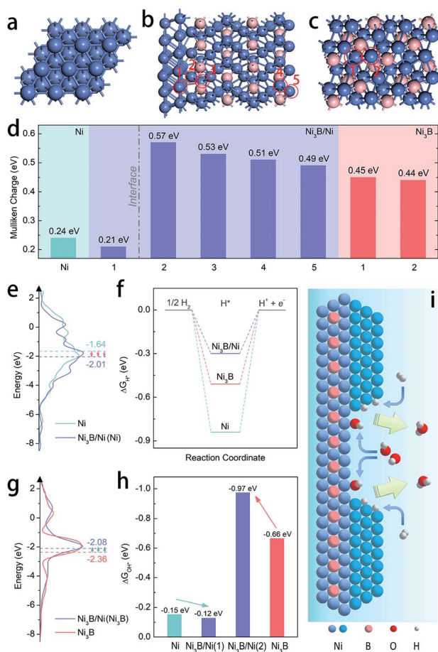
Fig. 4 Atomic structure diagrams of the optimized models of (a) Ni, (b) the Ni 3 B/Ni heterostructure, and (c) Ni 3 B. (d) Mulliken charges for hollow sites in Ni (111), 1–5 sites in the Ni 3 B/Ni heterostructure, and 1–2 sites in Ni 3 B (001), as marked by red circles in (b) and (c). (e) DOS plots of Ni and the Ni 3 B/Ni heterostructure (each d-band center is highlighted by a dashed line). (f) Free-energy diagram for H* adsorption on Ni, the Ni 3 B/Ni heterostructure, and Ni 3 B. (g) DOS plots of the Ni 3 B/Ni heterostructure and Ni 3 B (each d-band center is highlighted by a dashed line). (h) Free-energy diagram for OH* adsorption on Ni, the Ni 3 B/Ni heterostructure, and Ni 3 B. (i) Schematic illustration of the accelerated HOR process at the interface between Ni and Ni 3 B in the Ni 3 B/Ni heterostructure.
