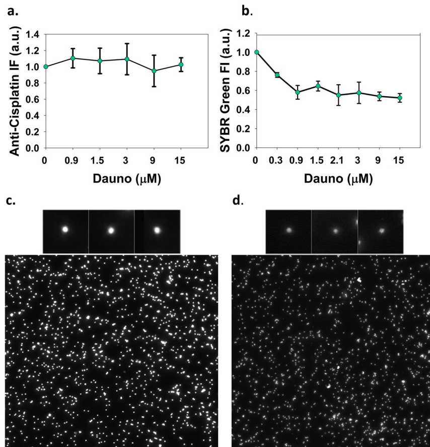
Figure 5. Effect of Dauno treatment of nuclei on the formation of Cis-Pt-DNA adducts. Agarose-embedded nuclei of HeLa cells co-treated with 40\ \mu\text{M} Cis-Pt and Dauno used at the concentrations indicated, for 16 hrs ( a,b ). The amount of all Cis-Pt-DNA adducts ( a ) and ICLs ( b ) were measured by LSC. ( a ) Total Cis-Pt-DNA adduct levels detected by indirect immunofluorescence using anti-Cisplatin primary and Alexa 488 conjugated secondary antibody on deproteinized nuclear halo samples. ( b ) ICL levels measured by SYBR Green I staining of double-stranded DNA. The nuclear halos were deproteinized after renaturation of the alkaline-denatured DNA strands and the undenatured DNA molecules were removed by S1 nuclease treatment. ( c,d ) Field-images of the LSC scans of alkaline halo samples in the case of nuclei treated with Cis-Pt only ( c ), or with Cis-Pt and 15\ \mu\text{M} Dauno ( d ). Fluorescence intensities are shown in arbitrary units (a.u.). Representative nuclei of each sample are shown in the insets. Error bars in panel a and b represent SEM values calculated based on two independent biological experiments, each in duplicate.
