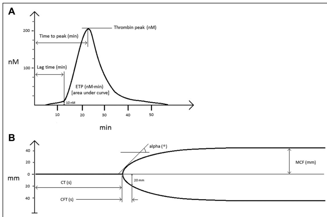
Figure 1. Exemplification of result curves of (A) plasma thrombin concentration in calibrated automated thrombogram (CAT) and (B) clot firmness in rotational thromboelastometry (ROTEM). Lag time indicates time from start until 10 nmol/L of thrombin is detected; time to peak, the time until maximal concentration is reached; peak, maximum concentration registered; ETP, endogenous thrombin potential—area under the curve; CT, clotting time; CFT, clot formation time; MCF, maximum clot firmness.
