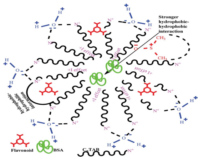
Fig. 23 Micellisation form of flavonoids in the aq-DMSO system.
