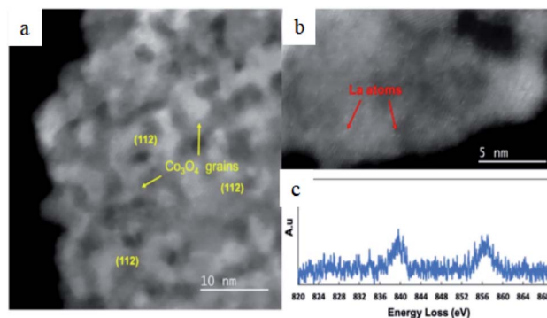
Fig. 11 (a) and (b) HAADF-STEM images of La/Co 3 O 4 , in which Co 3 O 4 nanocrystallites were marked by yellow arrows and La SACs were marked by red arrows. (c) EELS spectrum of La SACs. This figure has been reproduced from ref. 77 with permission from Cambridge University Press, copyright 2020.
