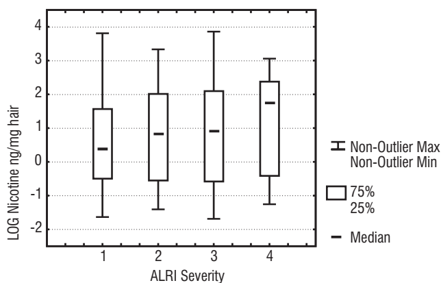
Figure 2. Box plot of hair nicotine levels according ALRI severity (only children with positive severity signs included).
