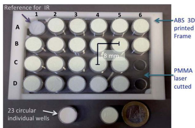
Fig. 9 The multi-well plate, its components and coordinates.
