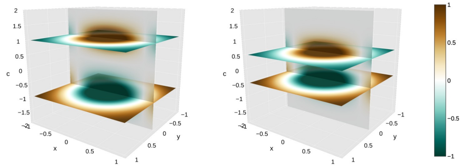
Fig 6. Connectivity kernel in 3D physical and color space. Left. W_1 defined with r_0 = 0 and c_0 = 1 . Right. W_2 defined with r_0 = 0 and c_0 = .5 . The color bar extends between -1 and 1 , going from dark green (negative values, strong inhibition) to dark orange (positive values, strong excitation). We provide an interactive 3D animation of the connectivity kernels \omega(r_0, c_0, \cdot, \cdot) for all values of c_0 \in \mathcal{C}_{opp} in S1 File. For varying r_0 , the kernel is just spatially translated along r_0 . However, for varying c_0 , the positive and negative gaussian kernels in f follow c_0 and -c_0 , collide when c_0 goes through zero, then exchange of position when |c_0| grows again.
