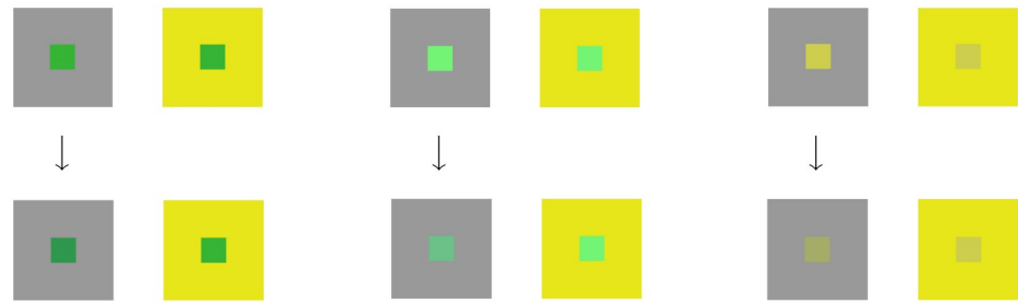
Fig 3. A typical color matching experiment. Upper row, left to right. For each of the three pairs of (gray, yellow) large squares, the central patches have identical colors. Their HSL coordinates are (120^\circ, 55\%, 46\%) , (120^\circ, 85\%, 71\%) , (60^\circ, 57\%, 56\%) , respectively. The HSL color space is extensively used in computer graphics and defined in [21]. Lower row, left to right. One of the authors (A.S.) has modified the HSL coordinates of the left central patch, in order to obtain perceptually equal patches (as much as possible). This is called matching . We can see how far the “perceived” HSL are from reality: (138^\circ, 55\%, 39\%) , (140^\circ, 41\%, 59\%) , (66^\circ, 29\%, 54\%) . The reader probably does not perceive the two patches as perceptually equal, because matching is subject-dependent.
