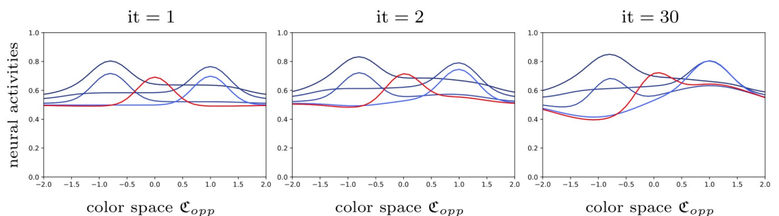
Fig 8. Dynamics of the color neural field Eq (3). The neural activities are plotted after a. one, b. two, c. thirty iterations, and convergence is reached after fifteen iterations. The red curve indicates the activity a_q^{test}(r_0, \cdot) of hypercolumn r_0 corresponding to the test stripe. Other blue curves correspond to spatial points r_i located on surrounding stripes. Notice that only four and not eight different curves are seen, because of the axial symmetry artificially introduced to facilitate numerical computations, as explained in S2 Appendix. A video of the dynamics is provided in S1 Video.
