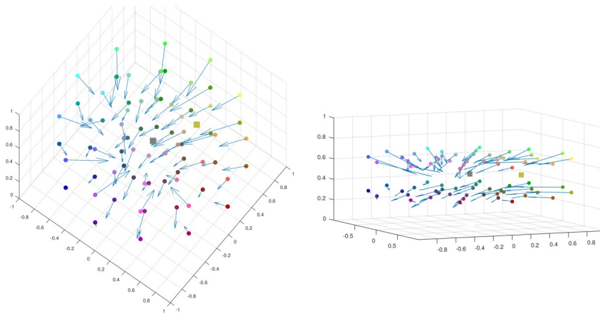
Fig 5. Yellow pushes towards blue. Using fixed Yellow test and Gray comparison surrounds (symbolized as squares in the figure) similarly to Fig 3, we obtain a vector field of shifts ( c^{test} , c^{match} ) in the HSL space (symbolized as spheres and arrows). There is clearly a “yellow pushes towards blue” phenomenon, where contrast wins.
