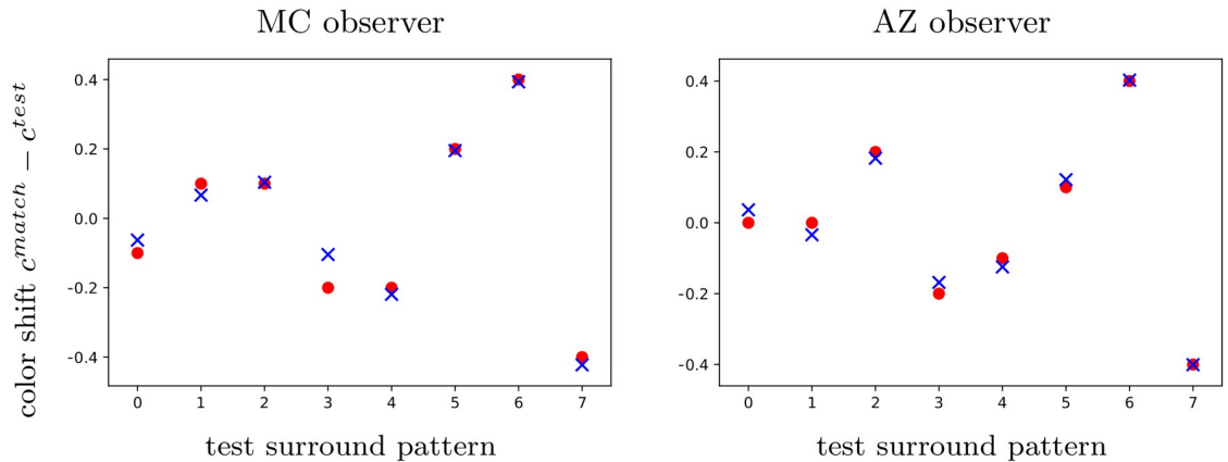
Fig 9. Our tuned model predicts color shifts from [18]. Left. Observer ‘MC’. Right. Observer ‘AZ’. Red dots indicate experimental data, while blue crosses stand for predicted matching comparison colors. The data has been averaged over three sets of experiments, as detailed in the original article. The ordinate corresponds to the color shift, expressed in \mathcal{C}_{opp} coordinates with c = s - 1 . The abscissa i = 0, \dots, 7 refers to the test pattern: p/p, l/l, p/w, l/w, w/p, w/l, p/l, l/p, where p stands for purple, l for lime, w for white.
