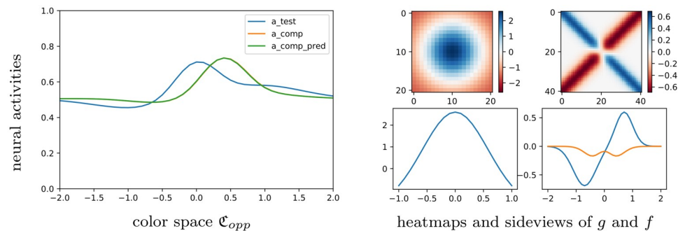
Fig 10. Comparing color sensations for real and predicted matching color. Left. Color sensations a_q^{test} , a_q^{comp}[c^{match}] and a_q^{comp}[c^{pred}] . Right. Functions f and g for the regressed parameter value q = q_{MC} . Right, up. Heatmaps for g and f . Right, down. Corresponding side views.
