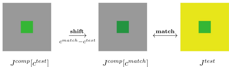
Fig 2. Color matching measures the influence of context over color perception. The green color c^{test} is tested against a yellow surround in the test image J^{test} . The observer changes the comparison color c^{comp} inside J^{comp} until a match occurs at c^{match} between the two central patches. Color induction is measured as the obtained shift.
