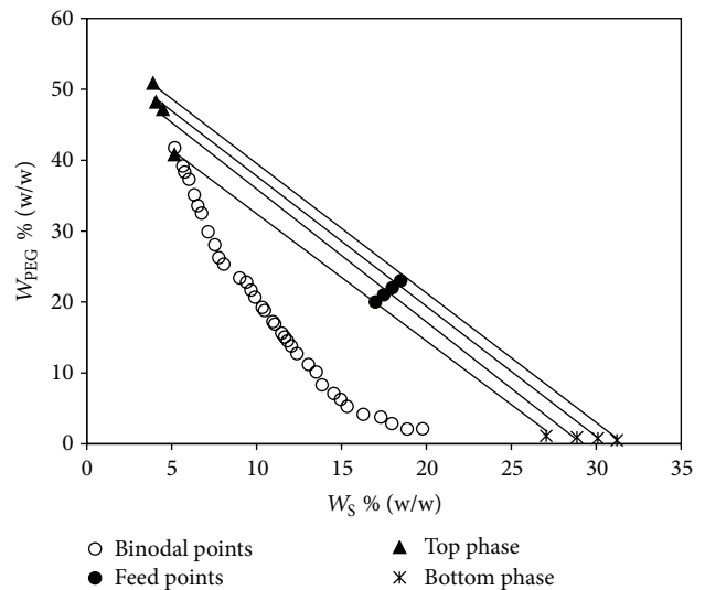
FIGURE 3: Binodal curve and tie lines for PEG 6000 ( W_{PEG} ) + sodium succinate ( W_S ) + water system at 318.15 K.
