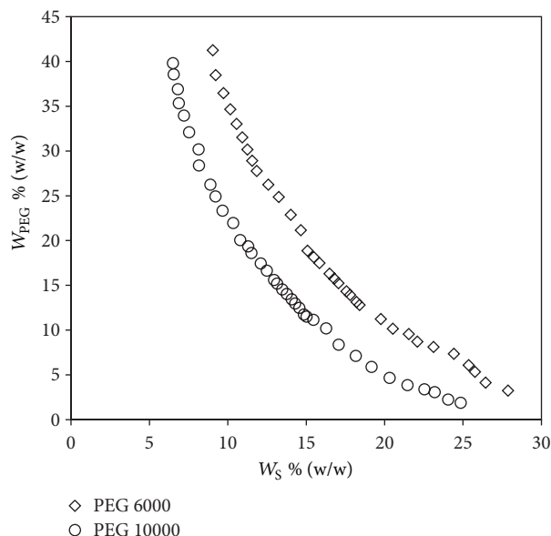
FIGURE 5: Effect of molecular weight of PEG on the binodal curve for the PEG ( W_{PEG} ) + sodium succinate ( W_S ) + water systems at 298.15 K.
