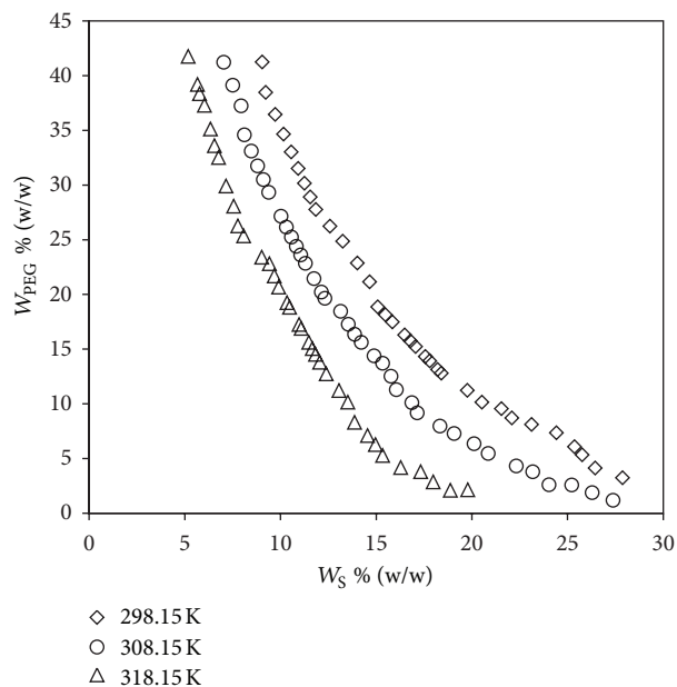
FIGURE 1: Effect of the temperature on the location of binodal curves for the PEG 6000 ( W_{PEG} ) + sodium succinate ( W_S ) + water systems.
