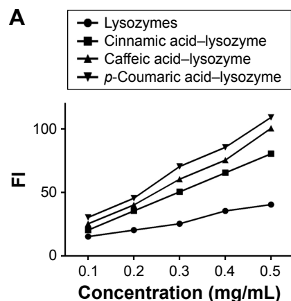
Figure 4 Surface-hydrophobicity index and secondary-structure stability of the four enzymes. Notes: (A) Correlation between FI index and concentration; (B) secondary-structure content of each group. Abbreviation: FI, fluorescence index.
