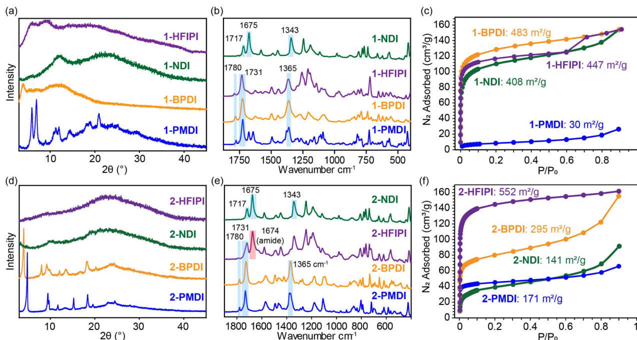
Fig. 1 (a) Overlay of PXR D patterns of 1-XDI MOFs. (b) Overlay of ATR-IR spectra of 1-XDI MOFs. Characteristic imide IR bands are highlighted in blue. (c) \text{N}_2 adsorption isotherms for 1-XDI MOFs measured at 77 K. (d) Overlay of PXR D patterns of 2-XDI MOFs. (e) Overlay of ATR-IR spectra of 2-XDI MOFs. Characteristic imide IR bands are highlighted in blue. (f) \text{N}_2 adsorption isotherms for 2-XDI MOFs measured at 77 K.
