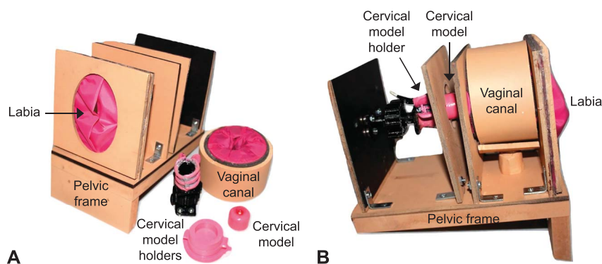
Fig. 1. Front (A) and side (B) view of the LUCIA model.
