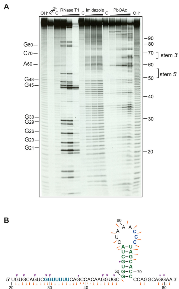
Figure 3. Structure probing of the 3' stem-loop. (A) RNA was 5'-end-labelled with [ \gamma - ^{33}\text{P} ] ATP and subjected to limited RNase or chemical cleavage using structure-specific probes. Sites of cleavage were identified by comparison with a ladder of bands created by limited alkaline hydrolysis of the RNA (OH ^- ; RNA heated to 100°C for 95 s [left lane] or 165 s [right lane]). Enzymatic probing employed RNase T1 (at 1, 10 and 100 U/mL) which preferentially cleaves after G bases in single-stranded regions. Chemical probing was with imidazole (2, 4 and 6 h exposure), or lead acetate (PbOAc; 10, 20 and 50 mM concentration in reaction), which show specificity for single-stranded regions. Uniquely cleaved nucleotides were identified by their absence in untreated control lanes (C). The regions corresponding to the 5' and 3' part of the stem-loop duplex are indicated. (B) The reactivities of RNase T1 (purple arrowheads) and imidazole (thin orange arrowheads) are indicated on a schematic of the TMEV PRF signal showing the evolutionarily conserved stem-loop structure (18). The size of the symbols is approximately proportional to the intensity of cleavage at that site.
