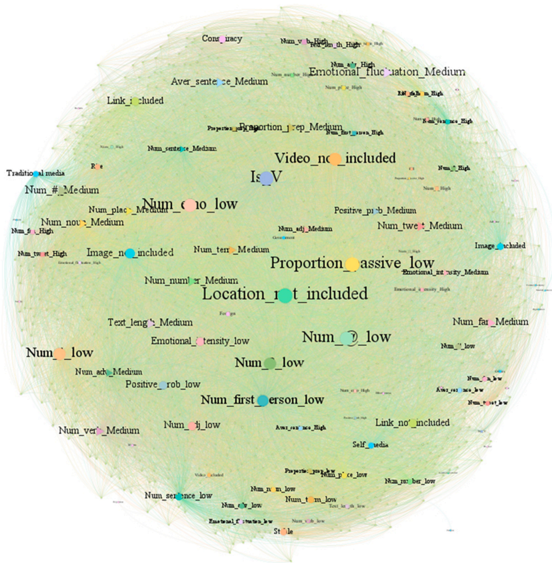
Fig. 9. “Disapprove” network.
