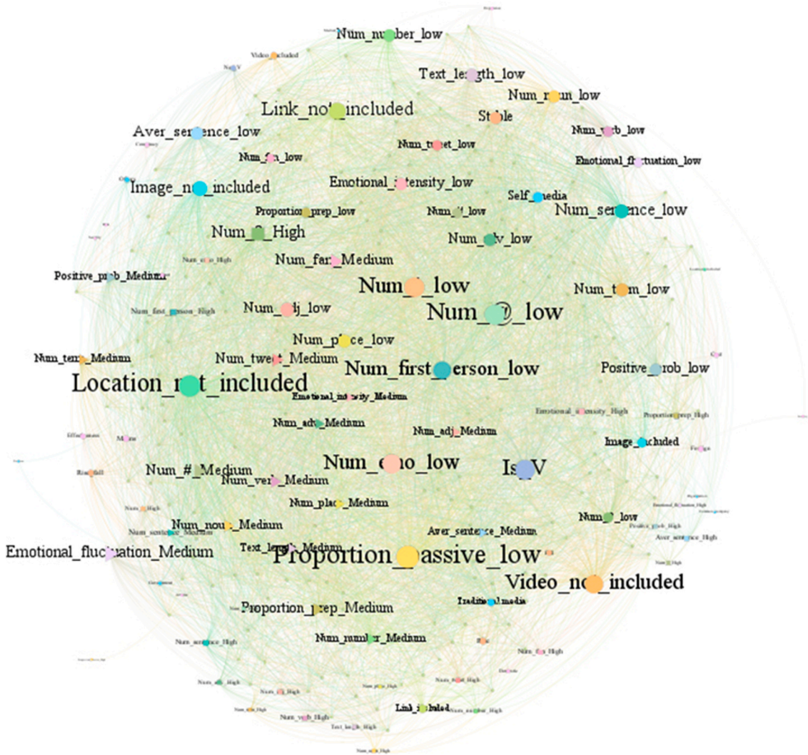
Fig. 10. “Unclear” network.
