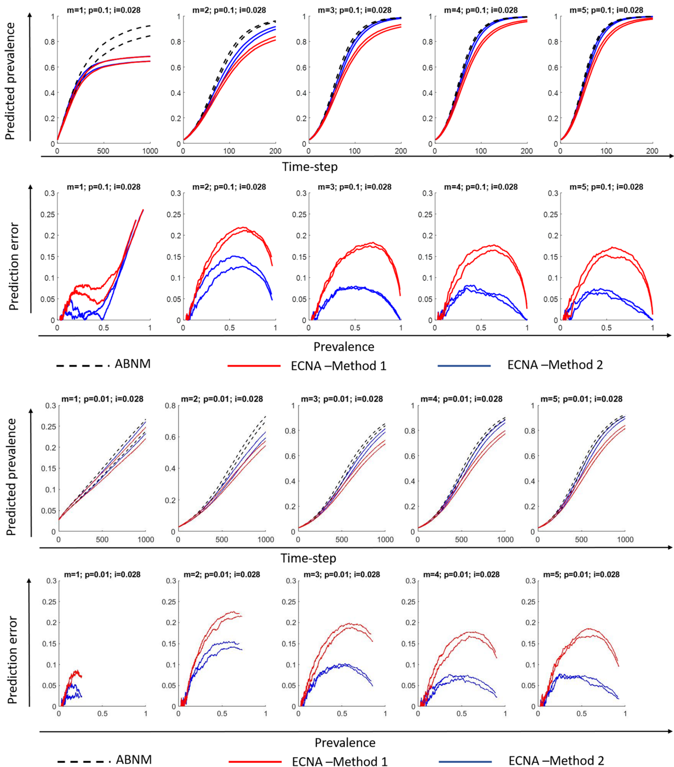
Fig. 3 Disease prevalence (proportion of population infected) predictions and prediction errors in ABENM (ECNA Methods 1 and 2) compared to ABNM for networks with minimum degree m = 1 to 5, transmission probability per exposure p = 0.1 and 0.01 , initial proportion infected i = 0.028 , and network size N = 10,000 ; Plots show the 5th and 95th percentile values of 100 runs. ABNM: Agent-based network model;
