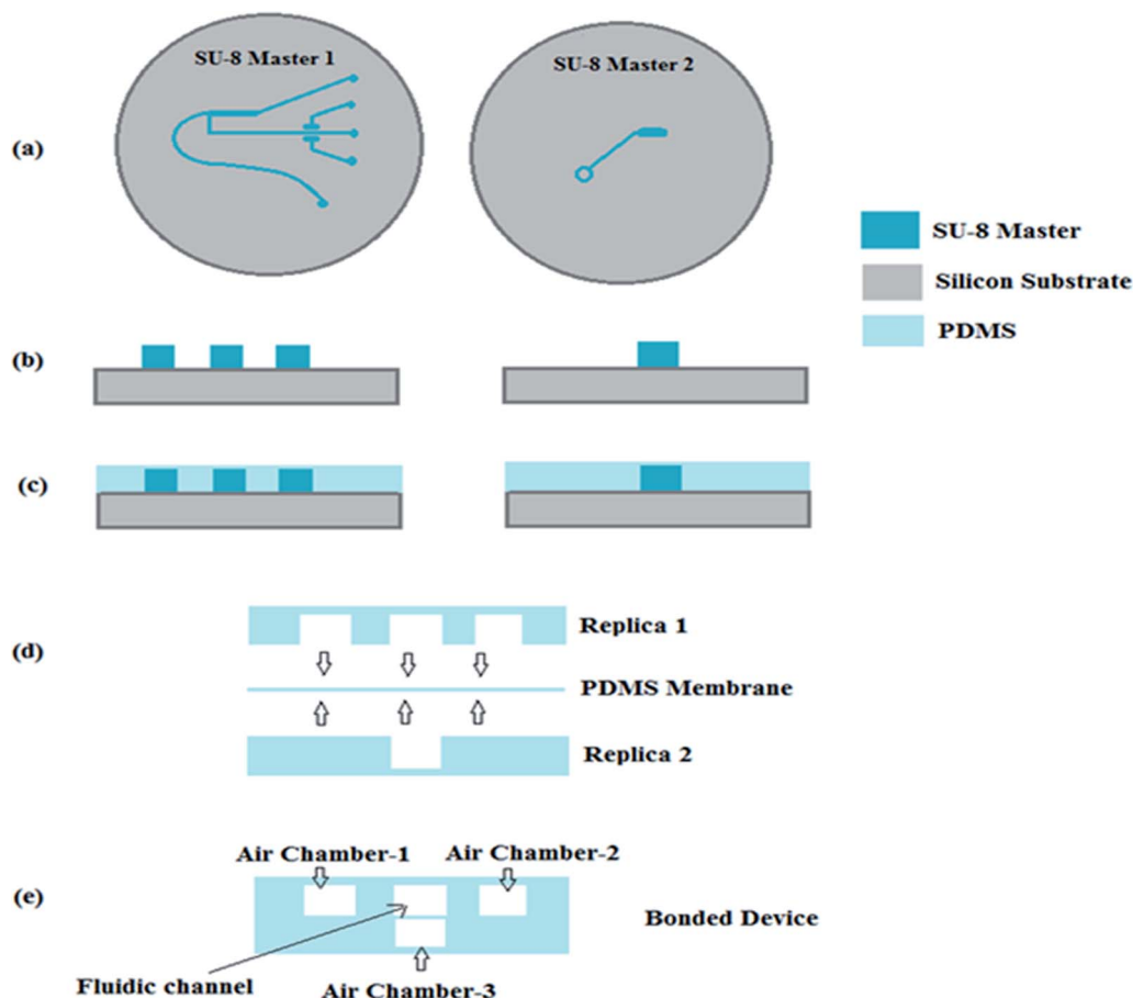
Fig. 4 Schematic diagram of the fabrication of the SU-8 masters of the microdevice's two component layers i.e. (a) the Layer 1 & 2 of SU-8 master and (b) the Layer 1 & 2 SU-8 master (side view); (c) casting of the mixture with a 10 : 1 ratio of PDMS pre-polymer and the curing agent and then the curing of this mixture at 120 °C for 20 minutes; (d) peeling off the PDMS Layer 1 and Layer 2 of the devices from the respective SU-8 masters and finally the bonding of both layers together with a PDMS membrane sandwiched in between these layers; (e) finally bonded microdevice with the designed fluidic channels and air chambers.
