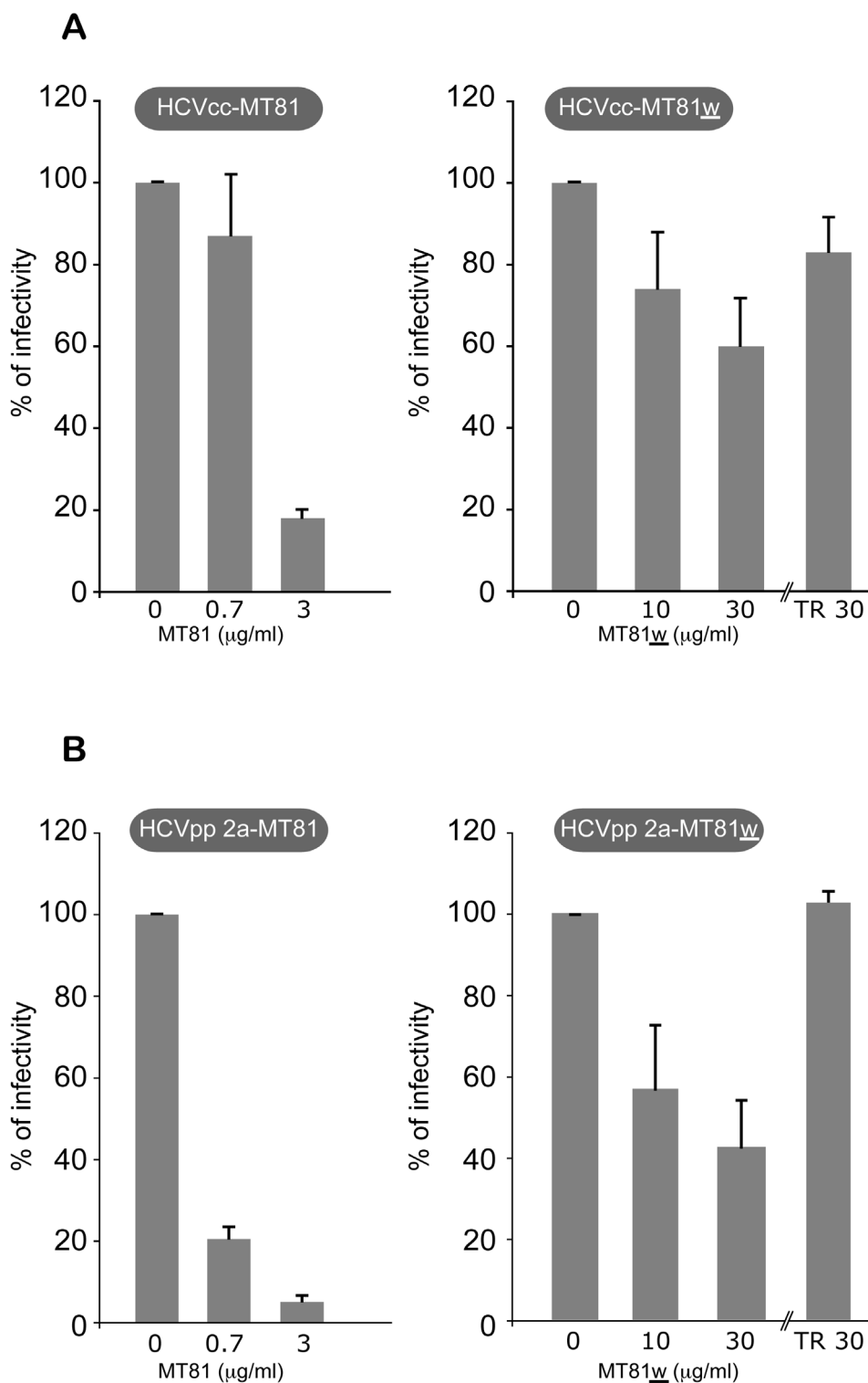
Figure 4 Neutralization assay of HCV infection with MT81 and MT81 w antibodies. HCVcc ( A ) and HCVpp 2a ( B ) infections of Huh-7w7/mCD81 cells were performed in presence of indicated concentrations of MT81 (left panels) or MT81 w (right panels) mAbs or in presence of 30 μg/ml of transferrin receptor (right panels, TR30). At 2 days post-infection, cells were lysed and processed as described in methods. P < 0.05 as calculated by the Mann-Whitney's test.
