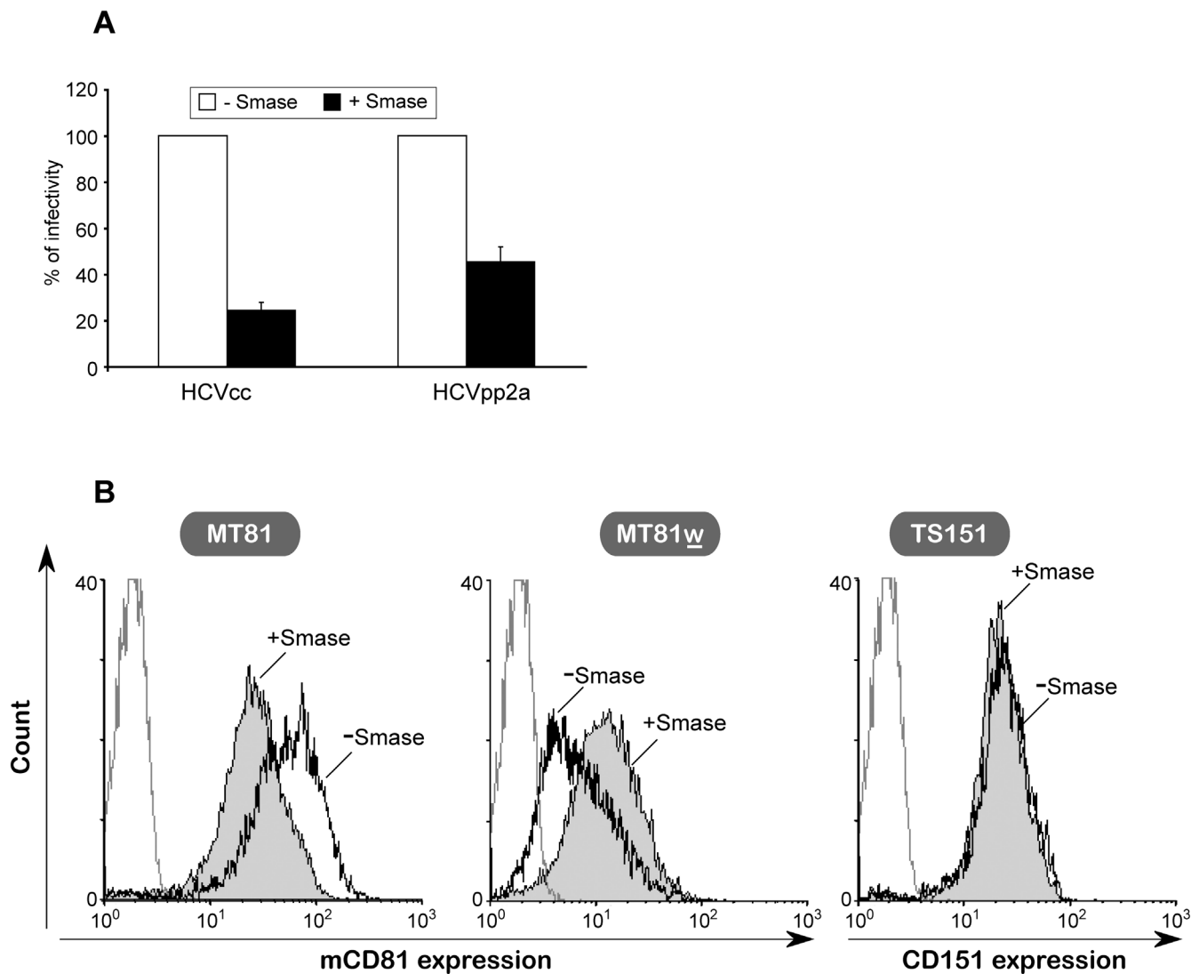
Figure 8 Ceramide enrichment of the plasma membrane of Huh-7w7/mCD81 cells inhibits HCV entry and increases association of CD81 with TEMs. A , Huh-7w7/mCD81 cells were pretreated (+Smase) or not (-Smase) with Smase prior to infection with HCVcc or HCVpp 2a. At 2 days post-infection, cells were lysed and processed as described in methods. P < 0.05 as calculated by the Mann-Whitney's test. B , Huh-7w7/mCD81 cells pretreated (+Smase) or not (-Smase) with Smase were stained with MT81 (left panel), MT81 w (middle panel) or TS151 (right panel) mAbs. Cells stained only with PE-conjugated secondary antibody were used as control (dotted line).
