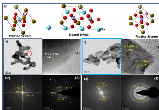
Fig. 12 (a) Unit cells (of pristine and doped perovskite oxides) generated from single point energy calculation using Gaussian, TEM micrographs [(b) (LSCF6482), (c) (BSCF6482)], high resolution -TEM images (b1 and c1), fast Fourier transform (FFT) pattern (b2 and c2) and SAED pattern (b3 and c3).
