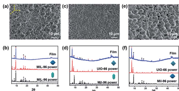
Fig. 3 SEM images and PXRD patterns of the mixed MOF films prepared using CH 2 Cl 2 as the casting solvent: (a and b) MIL-96 spindle morphology and hexagonal bifrustum morphology film; (c and d) MIL-96 spindle morphology and UIO-66 octahedral morphology film; (e and f) MIL-96 hexagonal bifrustum morphology and UIO-66 octahedral morphology film.
