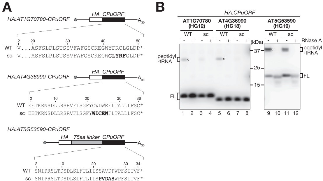
Figure 3. Effects of scrambling the CPuORF amino acid sequences on translation arrest. (A) Schematic representation of RNAs used for in vitro translation. The amino acid sequences of the WT and scramble (sc) mutant versions of the AT1G70780, AT4G36990, and AT5G53590 CPuORFs are indicated. The scrambled amino acids in the sc mutant sequences are shown in bold. (B) RNAs encoding the constructs shown in (A) were translated in WGE for 15 min. Translation products were treated with (+) or without (–) RNase A, and then separated by SDS-PAGE and immunoblotted with an anti-HA antibody. The positions of molecular mass standards and full-length translation products (FL) are indicated. The open arrowheads mark the WT CPuORF sequence-dependent peptidyl-tRNAs. For each panel, a representative result of two independent experiments is shown.
