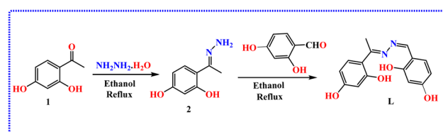
Scheme 1 Synthesis of chemosensor L .
