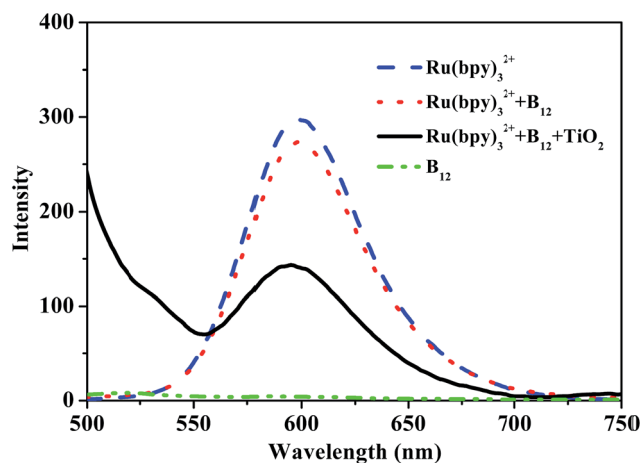
Fig. 10 The steady-state emission of Ru(bpy) 3 Cl 2 before and after adding [(CN)(H 2 O)Cob(III)7C 1 ester]Cl and TiO 2 in methanol. ([Ru(bpy) 3 Cl 2 ] = [(CN)(H 2 O)Cob(III)7C 1 ester]Cl] = 4.7 × 10 -5 mol L -1 , TiO 2 = 0.2 g L -1 , λ ex = 450 nm).
