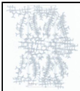
Fig. 2. The packing of (I), viewed down the c axis. H atoms not involved in hydrogen bonding have been omitted.
