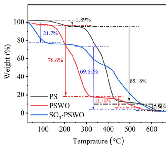
Fig. 6 Thermal stability analysis of PS, PSWO, and \text{SO}_3 -PSWO.
