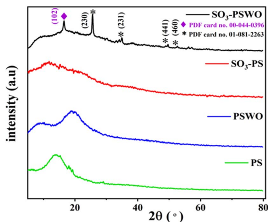
Fig. 5 XRD patterns of PS, PSWO, \text{SO}_3 -PS, and \text{SO}_3 -PSWO.
