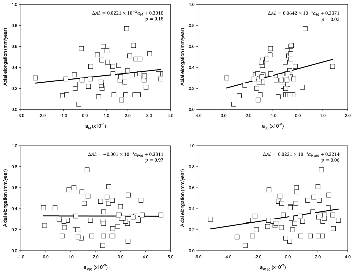
FIGURE 4. Relationship between the fitted first coefficients of RPRES and \Delta AL . Top left: a_M . Top right: a_{J0} . Bottom left: a_{P90} . Bottom right: a_{P(180)} .
