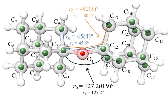
Figure 1. Experimentally determined r_0 structure (green spheres for carbon and red for oxygen) and computed one ( r_{cr} underlying structure, B3LYP-D3(BJ)/def2-TZVP) for the DAE monomer. Experimentally determined bond lengths are summarized in Table S3 in the Supporting Information.
