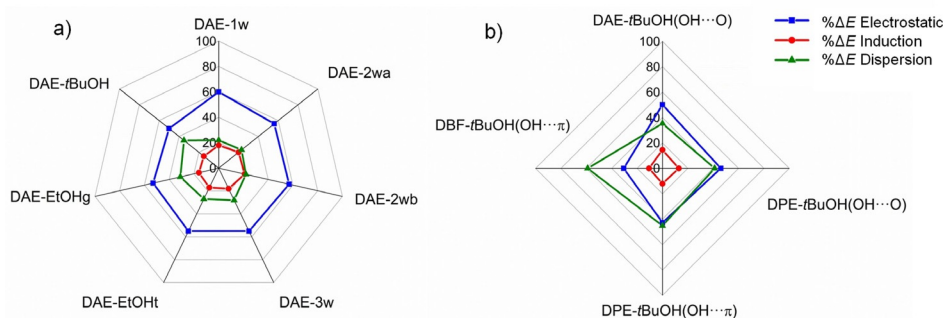
Figure 5. Radar charts showing the attractive contributions obtained from SAPT(0) computations as a percentage of the overall attractive interactions for DAE complexes in comparison to related t BuOH complexes. Electrostatics, induction, and dispersion contributions are shown in blue, red, and green, respectively.
