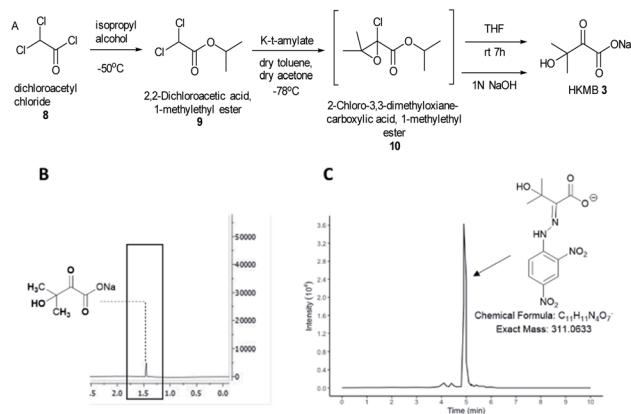
Fig. 2 (A) An optimised synthesis scheme towards HMKB 3 starting from dichloroacetyl chloride 8, via isopropyl 2-chloro-3,3-dimethylloxianoate 10 as a transit intermediate. (B) 1 H-NMR of 3 confirming the presence of the compound. (C) Extracted ion chromatogram (EICs) from LC-MS analysis of 3-DNPH.
