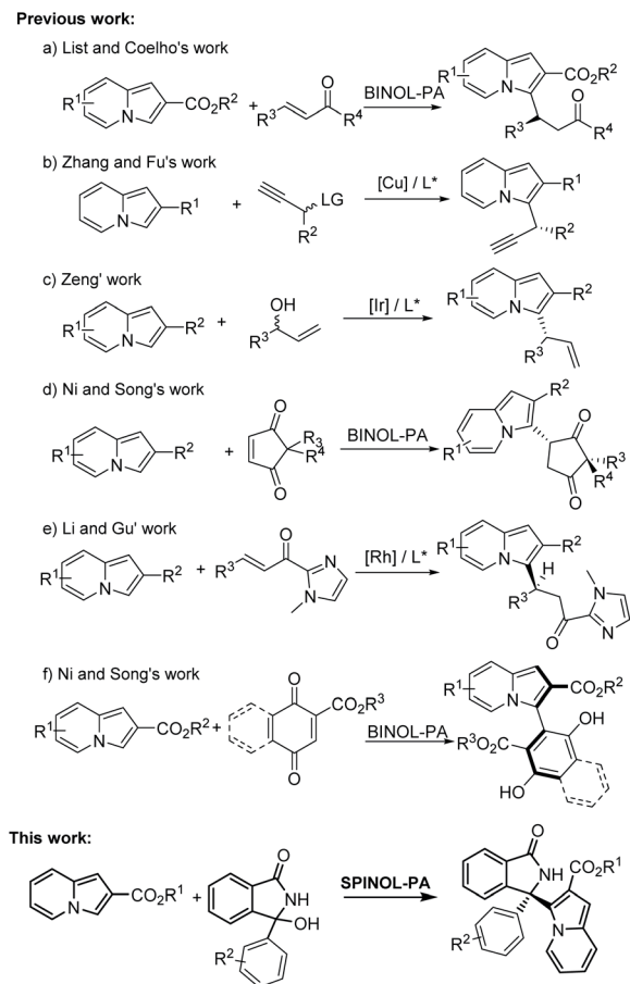
Scheme 1 Asymmetric functionalization of indolizines.
