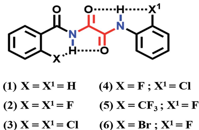
Scheme 1 The chemical structure of N^1 -benzoyl- N^2 -phenyl oxamide and its derivatives. The molecules, 1–6, differ in their substituents, X and X^1 , as shown in the scheme. In these molecules the formation of a HB results in a 6-membered ring with the NH(1) proton and a 5-membered ring with the NH(2) proton.
