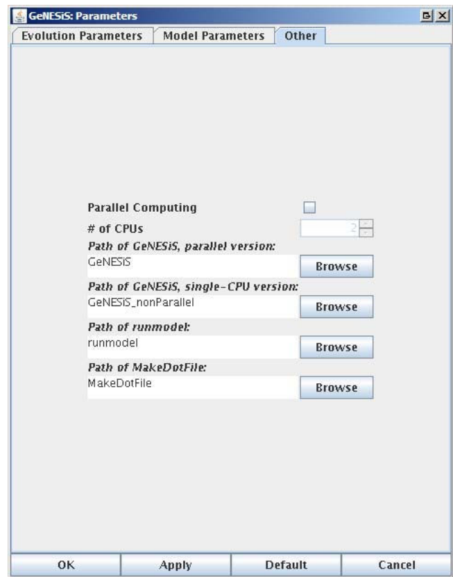
Figure 5 The parameters panes: Other Parameters.
