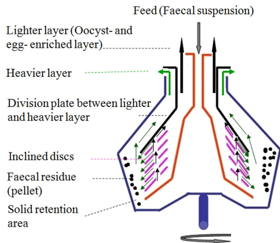
Figure 3. Schematic drawing of the centrifugal separation process.
