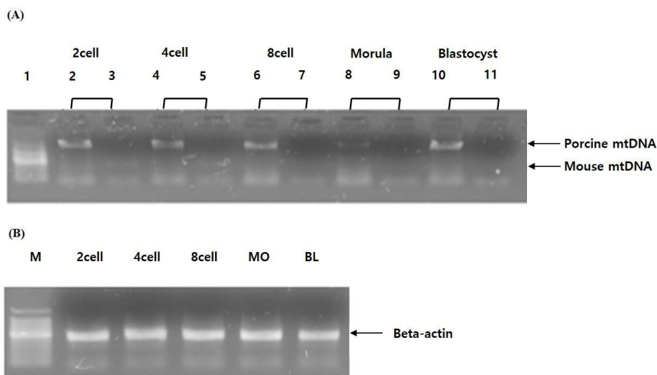
Fig. 2. mtDNA and mouse beta-actin DNA in mouse-porcine cloned embryos detected by PCR using species-specific primer pairs. (A) Lane 1: DNA marker. Lanes 2, 4, 6, 8, 10: The presence of porcine mtDNA (1,452 bp) in a mouse-porcine cloned embryo. Lane 3, 5, 7, 9, 11: The presence of mouse mtDNA (432 bp) in a mouse-porcine cloned embryo. (B) Mouse beta-actin (452 bp) in a mouse-porcine cloned embryo. M, marker; MO, morula; BL, blastocyst; mtDNA, mitochondrial DNA; PCR, polymerase chain reaction.
