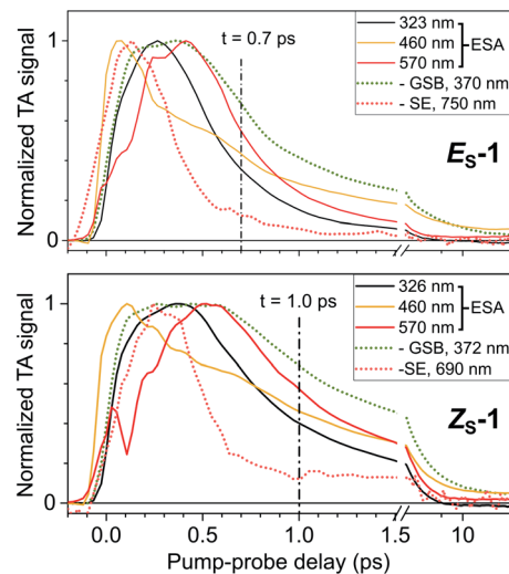
Fig. 4 Comparison of selected, normalised kinetic traces for methanol solutions of E_S -1 (top panel) and Z_S -1 (bottom panel). The kinetics of the UV ESA is illustrated at its absorption maximum of 323 nm ( E_S -1) or 326 nm ( Z_S -1). The Vis ESA kinetics are monitored at 460 nm (absorption maximum) and 570 nm (low-energy side). The GSB and SE kinetics are monitored by plotting the opposite of the negative signals observed at 370 nm ( E_S -1) or 372 nm ( Z_S -1), and 750 nm ( E_S -1) or 690 nm ( Z_S -1), respectively, to facilitate comparison with the other kinetic traces.
