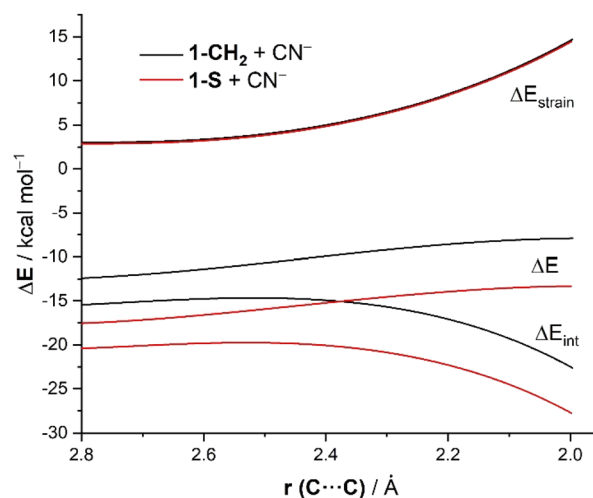
Fig. 1 Comparative ASDs of the reaction between \text{CN}^- and 1-CH 2 (black lines) and 1-S (red lines) projected onto the \text{C}\cdots\text{C} bond-forming distance and referred to the isolated reactants. All data have been computed at the ZORA-M06-2X/TZ2P//M06-2X/6-311+G* level.
