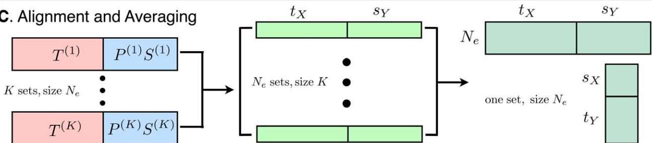
Figure 1. Schematic for the BICAR algorithm. This diagram illustrates the change in size and number of matrices during the steps of BICAR. A. During the decomposition step, both the temporal data X and spatial data Y are decomposed into K sets of N_e sources, where N_e \leq \min(s_X, t_Y) . The other necessary assumptions, t_X > t_Y and s_Y > s_X , are also schematically depicted. B. The matching step can be viewed as a concatenation, in which K sets of N_e super-sources and corresponding mixing elements are obtained. This step calculates permutations of the spatial decompositions to give the groupings. C. In the alignment step, the K sets of N_e matched sources are sorted into N_e sets of K super-sources and their corresponding mixing matrices. Here K < N_e , but there need be no particular relationship between these two quantities. Finally, after averaging and reproducibility calculations, matrices whose sizes correspond exactly with one of the X decompositions and one of the Y decompositions shown in A remain. doi:10.1371/journal.pone.0050268.g001
