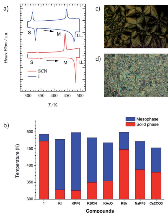
Fig. 1 Phase transition behaviour of M^+(\mathbf{1})\cdot X^- salts and the formation of the \text{Col}_h phase. (a) DSC profiles of K^+(\mathbf{1})\cdot\text{SCN}^- (red) and K^+(\mathbf{1})\cdot\text{I}^- (blue). (b) Temperature ranges of the solid phase (red) and \text{Col}_h phase (blue). POM images of the \text{Col}_h phase of (c) K^+(\mathbf{1})\cdot\text{I}^- at 483 K and (d) K^+(\mathbf{1})\cdot\text{SCN}^- at 473 K.
