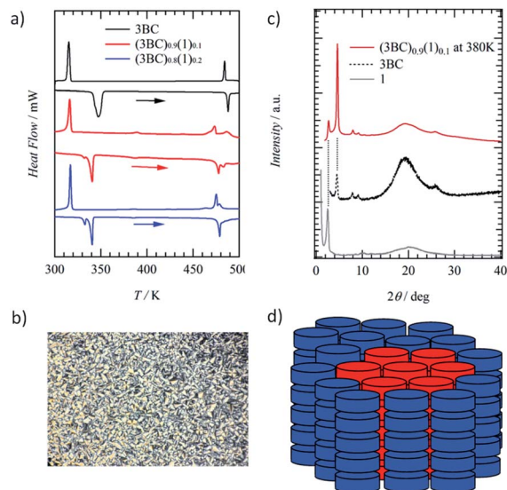
Fig. 3 Phase transition and mixed state of ionic channel (1)_\infty and ferroelectric (3\text{BC})_\infty in the \text{Col}_h phase. (a) DSC profiles of the mixed \text{Col}_h liquid crystal of (3\text{BC})_x(1)_{1-x} with x = 1, 0.9 , and 0.8 . (b) POM image of (3\text{BC})_{0.9}(1)_{0.1} at 450 K. (c) PXRD profiles of the \text{Col}_h phases of (3\text{BC})_{0.9}(1)_{0.1} at 380 K, 3BC at 380 K, and 1 at 380 K. (d) Schematic of the phase separation state of the ferroelectric 3BC domain (blue columns) and ionic channel 1 domain (red columns).
