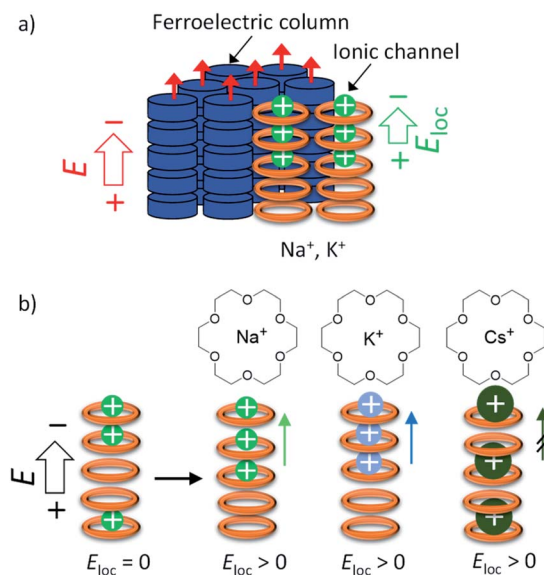
Scheme 2 Coupling between the ferroelectricity of 3BC and M + -inclusion (M + ) 0.5 (1) in the mixed Col h phase of (3BC) 0.9 [(M + ) y ·(1)·(X - ) 0.1 ] salts with M + = Na + , K + , and Cs + . (a) Coexistence of the ferroelectric domain of 3BC (blue column) and ionic channel of (M + ) y ·(1)·(X - ) 0.1 ; M + X - = Na + PF 6 - , K + PF 6 - , and Cs + (CO 3 2- ) 0.5 . The ionic conduction along the electric field ( E ) generates a local electric field ( E loc ) along the columnar direction. (b) 50%-occupied (M + ) 0.5 [[18]crown-6) ionic channels of (Na + ) 0.5 [[18]crown-6), (K + ) 0.5 [[18]crown-6), and (Cs + ) 0.5 [[18]crown-6) under electric field E .
