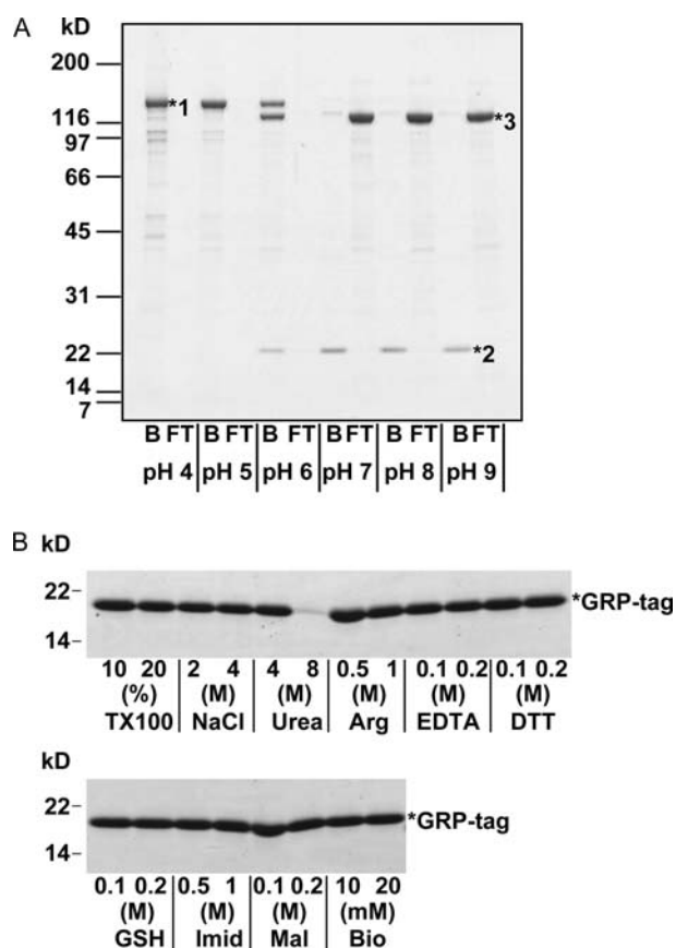
Fig. 4. Chemical stability of the complexes of the GRP-tag and the curdlan beads. (A) The stability of the GRP-tag–curdlan complexes between pH 4 and 9. GRP-RIG-I solubilized in a buffer at a pH of 4, 5, 6, 7, 8 and 9 was mixed with the curdlan beads, respectively. The beads of the each sample were washed with the same buffer and the remaining GRP-RIG-I on the beads was digested with GST-HRV 3C protease. After digestion, the proteins on the beads (Lane B) and in the flow-through of the beads (FT) were analyzed by SDS-PAGE. *1, GRP-RIG-I; *2, GRP-tag; *3, RIG-I. (B) The stability of the GRP-tag–curdlan complexes in the presence of chemical compounds generally used in protein purification. The complexes of the GRP-tag with the curdlan beads were mixed with the solutions as indicated in Table I and further washed with the same solutions, respectively. The residual complexes on the beads after washing were analyzed by SDS-PAGE.
