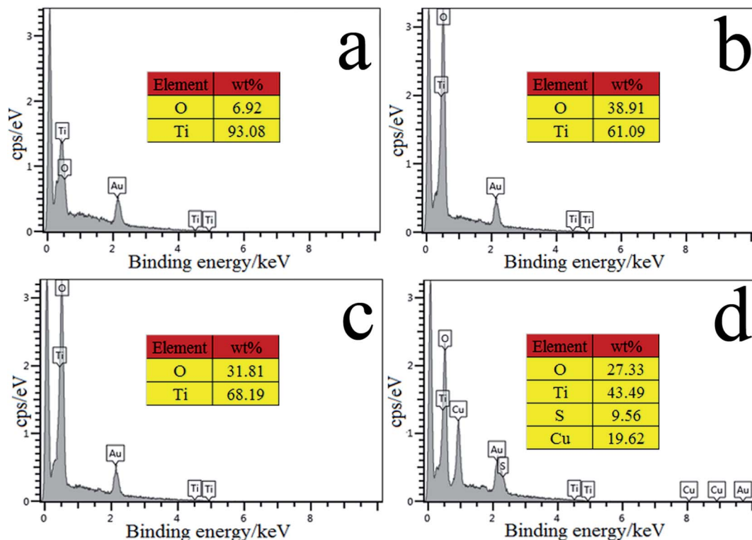
Fig. 3 EDS spectra of the untreated Ti wire (a), the \text{TiO}_2\text{NPs} (b), the fiber obtained after annealed \text{TiO}_2\text{NPs} (c) and the \text{CuS@TiO}_2\text{NPs} coated fiber (d).
