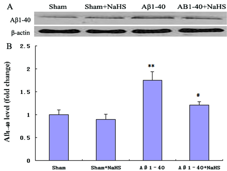
Figure 3 NaHS pre-treatment reduces Aβ 1-40 levels. Aβ 1-40 rats were treated with NaHS (5 mg/kg i.p. once daily). (A) Western blot of Aβ 1-40 protein contents. In hippocampal area CA1 the basal levels of Aβ 1-40 peptides decreased significantly after NaHS treatment. (B) The relative optical density was normalized to β-Actin. Results are expressed as mean ± S.E.M. with five rats in each group. ** P < 0.01 vs. sham; # P < 0.05 vs. Aβ 1-40 .
