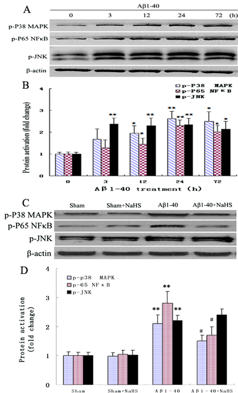
Figure 6 Western blotting analysis of the relative protein contents. (A, C) Western blot of various protein contents for phospho-p38 MAPK, phospho-p65 NFκB, and phospho-JNK. (B, D) The relative optical density was normalized to β-Actin. Data are mean ± S.E.M., n=4. **P < 0.01 *P < 0.05 vs. sham(control); #P < 0.05 vs. Aβ 1-40 .
