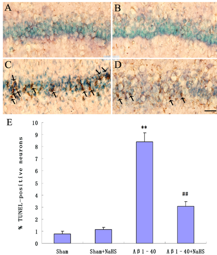
Figure 2 Effects of NaHS on DNA fragmentation in the hippocampus of rats injected with Aβ 1-40 . (A, B) No TUNEL-reactive cell was detected in the hippocampus from sham and sham + NaHS rats. (C) The significant number of degenerating pyramidal neurons, labeled with the TUNEL technique was observed in the CA1 subfield of the hippocampus. (D) The number of TUNEL-positive neurons significantly decreased in the hippocampus from Aβ 1-40 -injected rats receiving NaHS. Scale bar: 40 μm. Arrows point to degenerating pyramidal neurons with their nuclei stained with TUNEL technique. (E) Quantitative analysis of % TUNEL-positive neurons. Data are given as mean ± S.E.M. ** P < 0.01 vs. sham; ## P < 0.01 vs. Aβ 1-40 .
