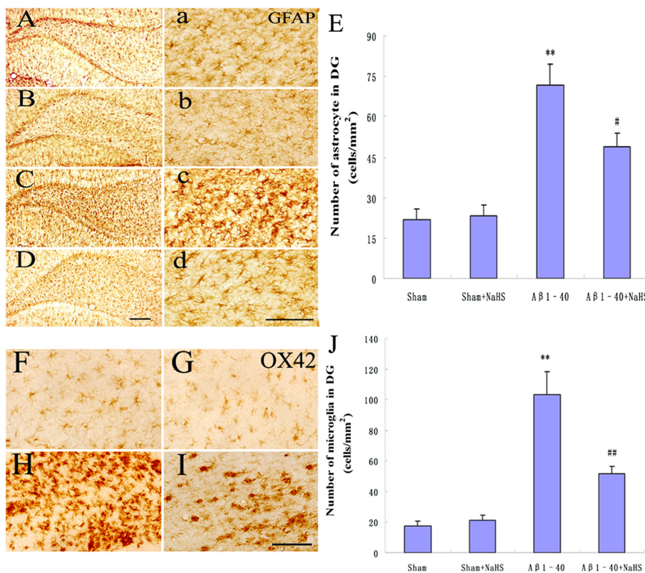
Figure 4 Effect of NaHS on Aβ 1-40 -induced the activation of glia in the DG region of rat hippocampus. (A-E, a-d) The distribution and number of GFAP-immunoreactive astrocytes in sham, sham + NaHS, Aβ 1-40 , and NaHS + Aβ 1-40 rats. Scale bar, 500 μm (A-D) and 50 μm (a-d). (F-J) Representative photographs and number of OX-42-immunopositive cells in sham, sham + NaHS, Aβ 1-40 , and NaHS + Aβ 1-40 rats. Scale bar: 250 μm. Six tissue sections per rat were used for the analysis ( n = 8-10). Data are presented as the mean ± S.E.M. ** P < 0.01 vs. sham; ## P < 0.01, # P < 0.05 vs. Aβ 1-40 .
