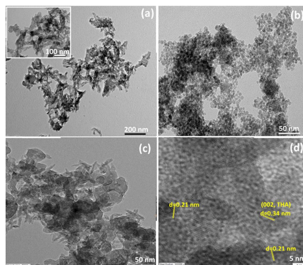
Fig. 2 TEM images of the (a) multi-trace elements co-doped apatite ( \text{Ca}_{10-6}\text{M}_6(\text{PO}_4)_{5.5}(\text{CO}_3)_{0.5}(\text{OH})_2 , \text{M} = trace elements, THA), (b) magnetic Mn–Zn nanoferrite ( (\text{Mn}, \text{Zn})\text{Fe}_2\text{O}_4 particles, BioMags) and THAiBioMags nanoparticles at low (c) and high (d) resolution, respectively.
